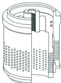
Figure 8 - Q-Cage™ and Q-Cage™ Level 2 Trim
