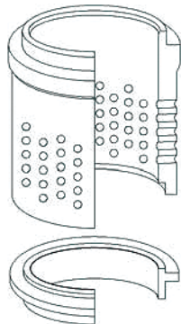
Figure 7 - Flash-Flo® Trim
