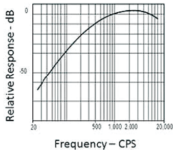
Figure 1, Ref. 1 - A weighting filter network
