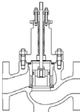
Figure 14 - Globe Valve, Hastelloy C, Dual Seal Bonnet
