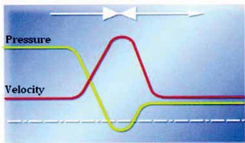
Figure 4 - Cavitating Service
