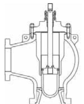
Figure 25 - V701 18x20 Digester Tail Valve
